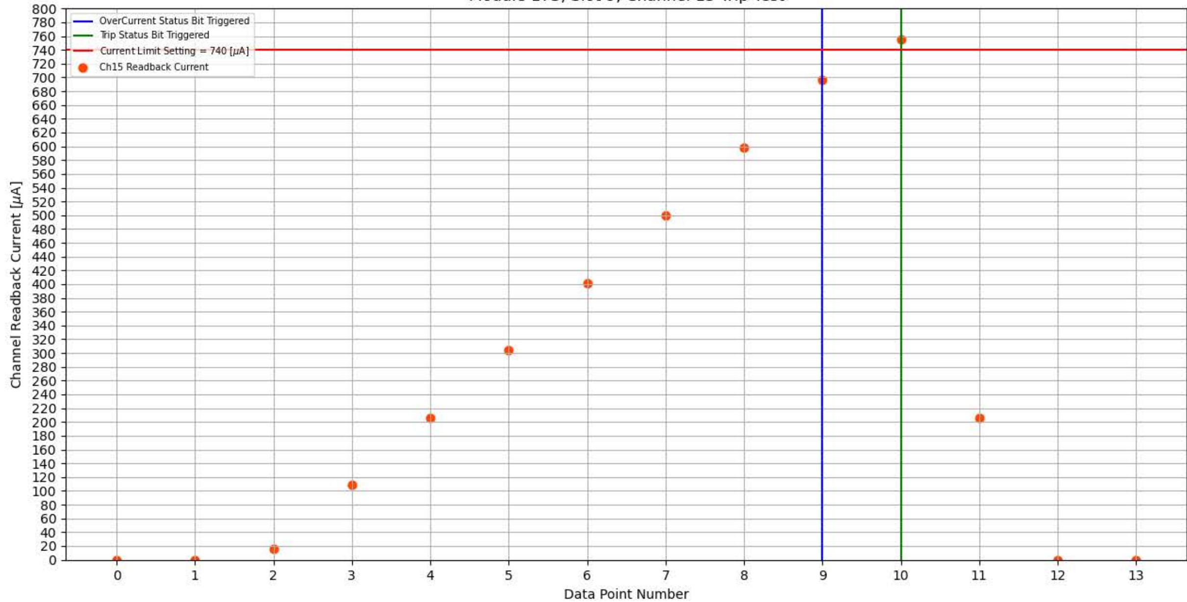
Module 173, Slot 9, Channel 15 Trip Test
