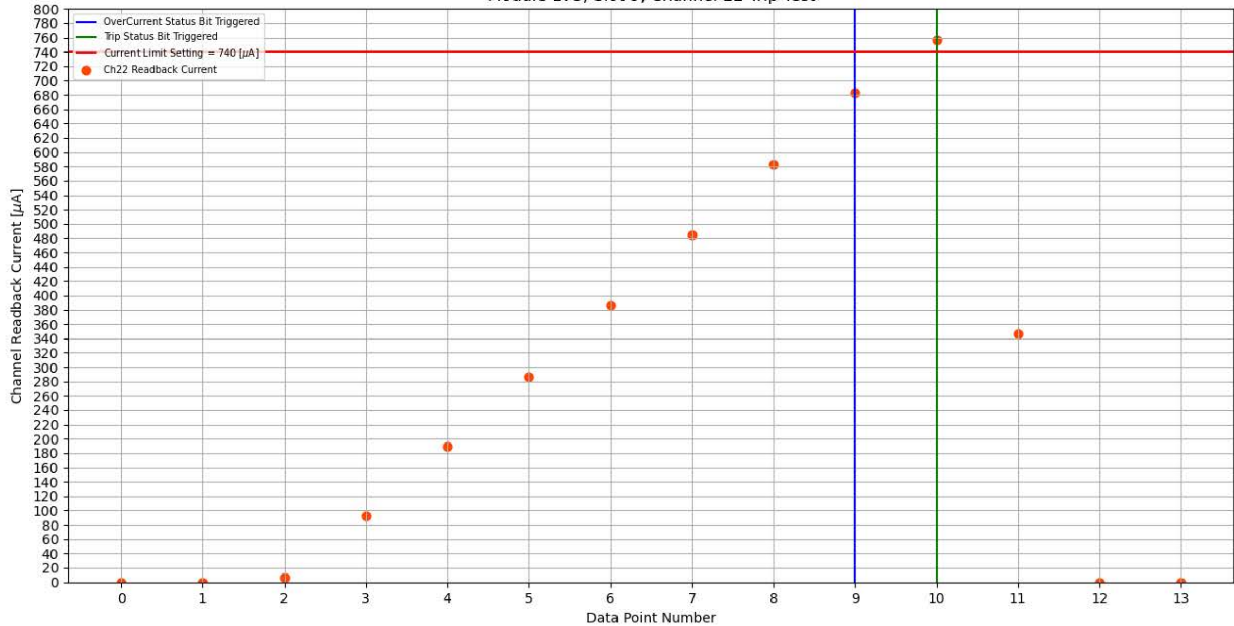
Module 173, Slot 9, Channel 22 Trip Test
