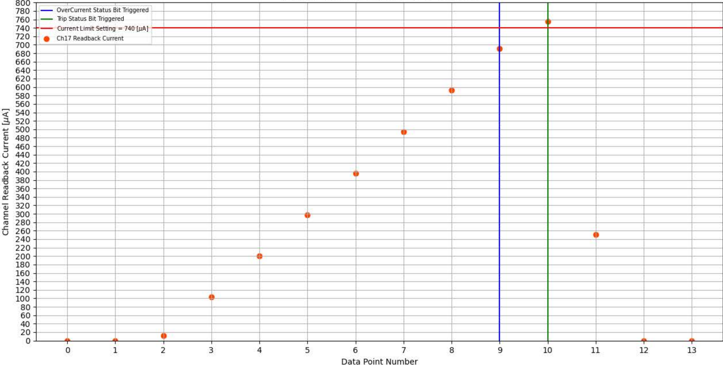
Module 173, Slot 9, Channel 17 Trip Test
