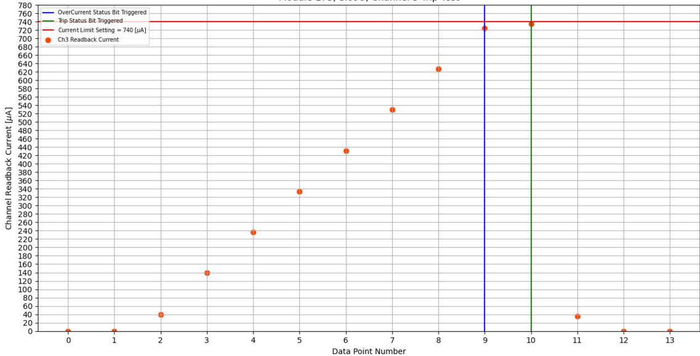
Module 173, Slot 9, Channel 3 Trip Test
