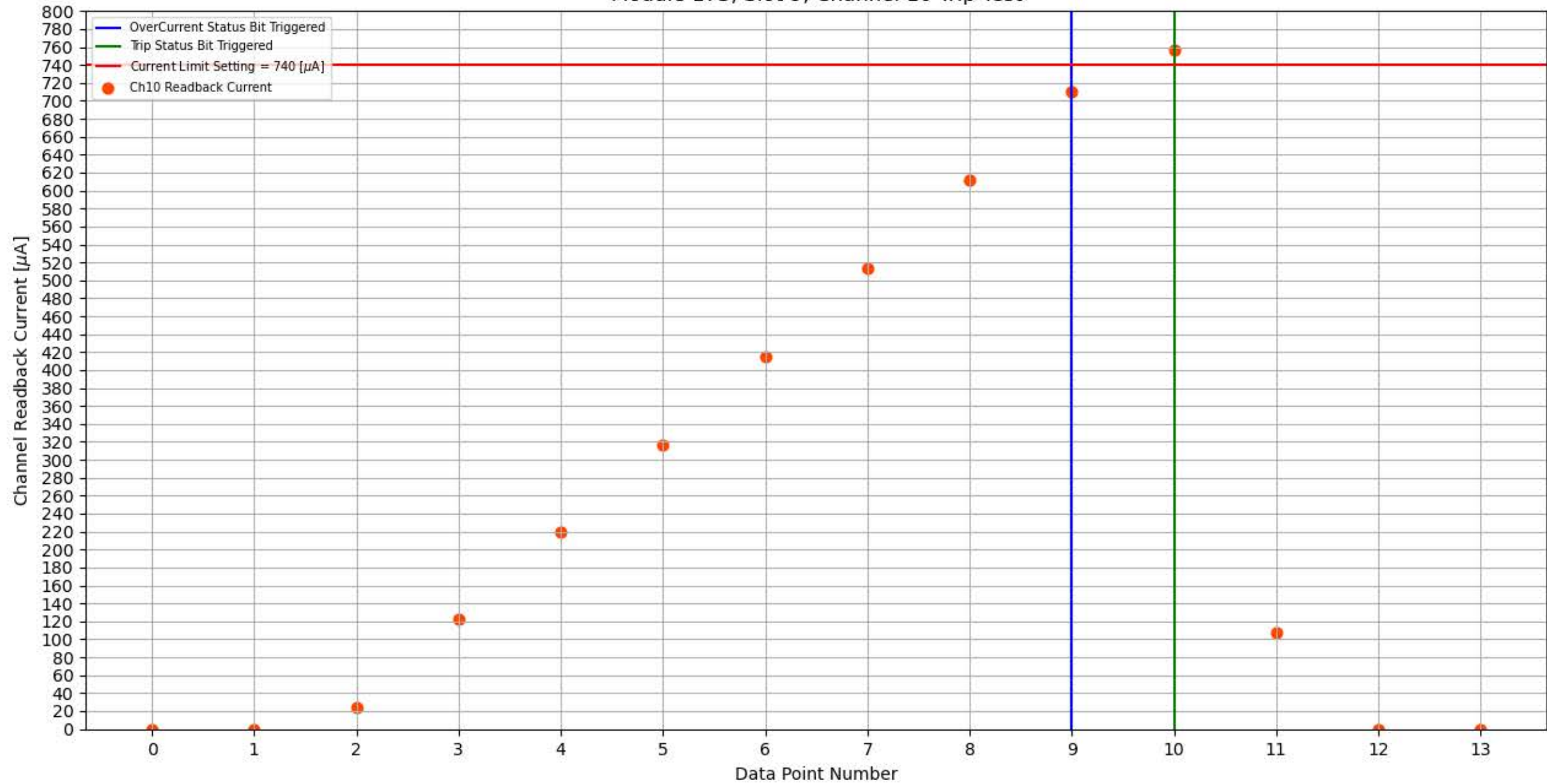
Module 173, Slot 9, Channel 10 Trip Test
