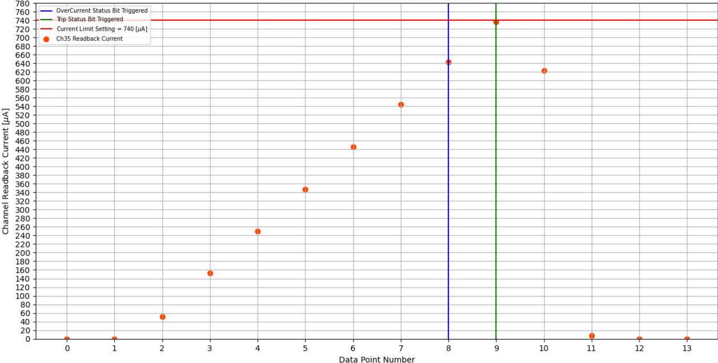
Module 173, Slot 9, Channel 35 Trip Test
