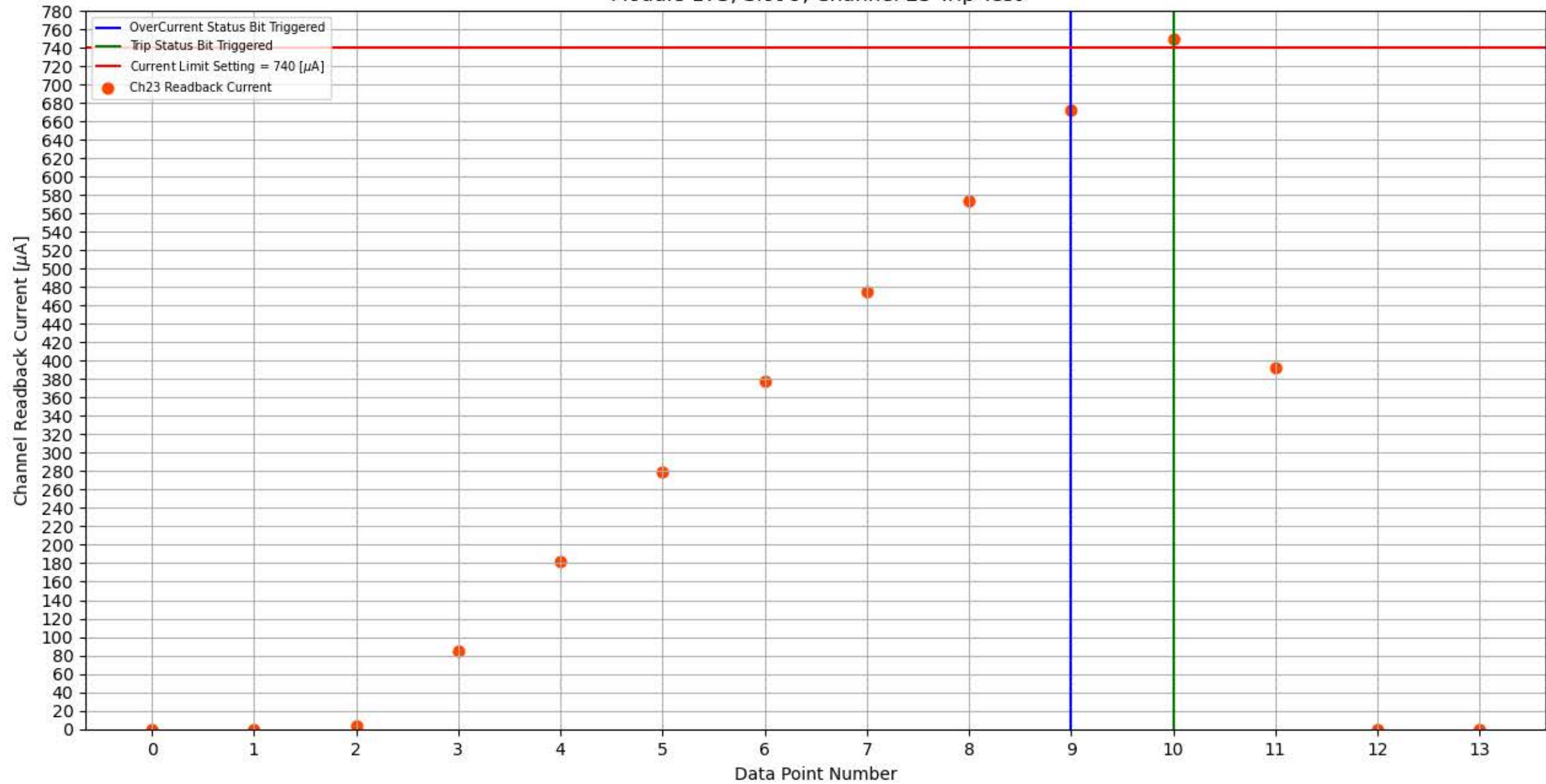
Module 173, Slot 9, Channel 23 Trip Test
