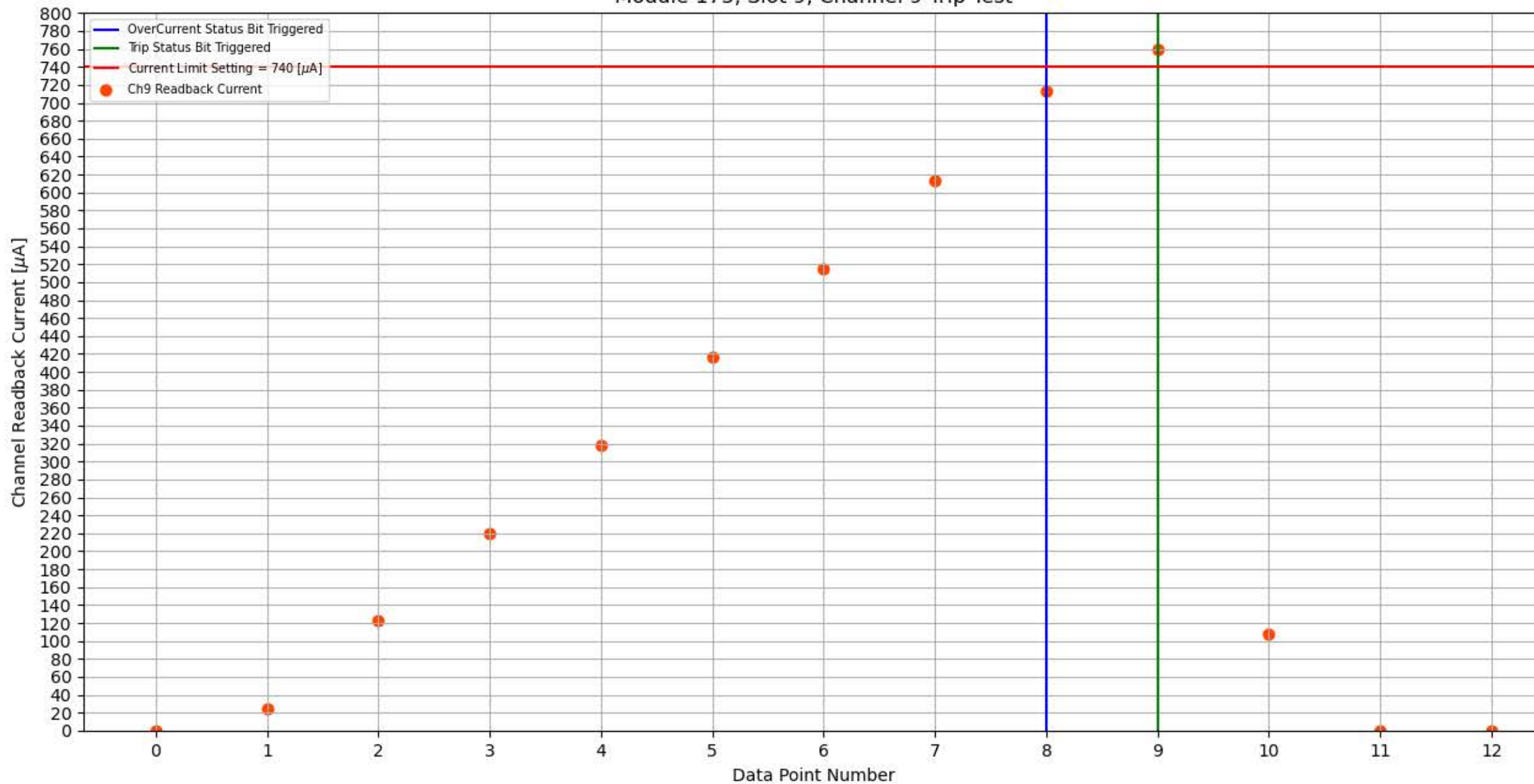
Module 173, Slot 9, Channel 9 Trip Test
