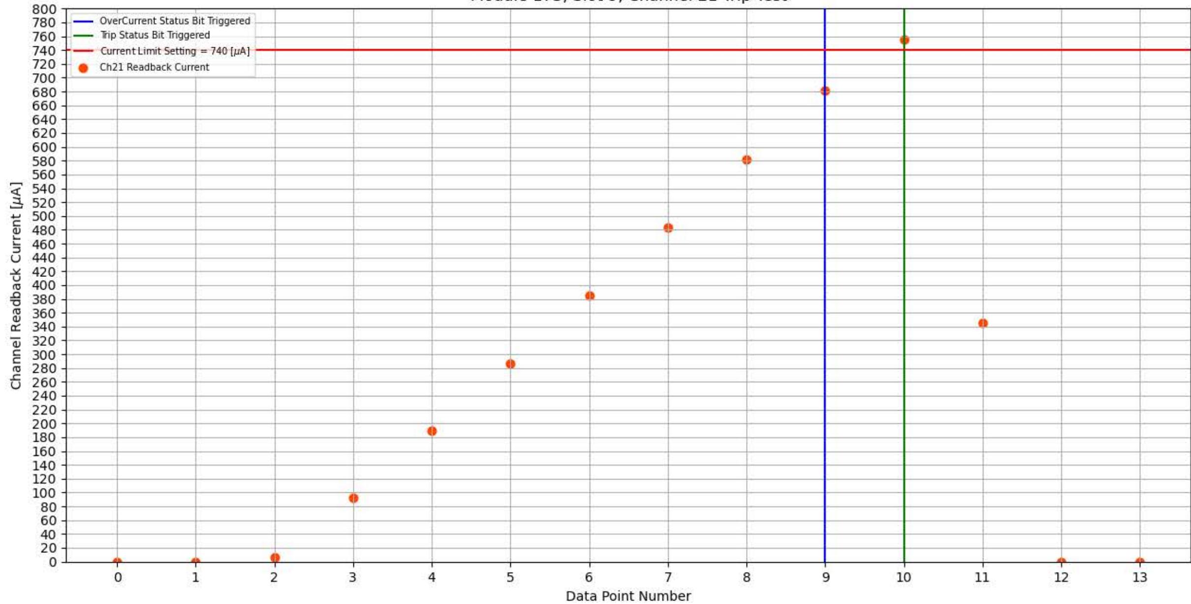
Module 173, Slot 9, Channel 21 Trip Test
