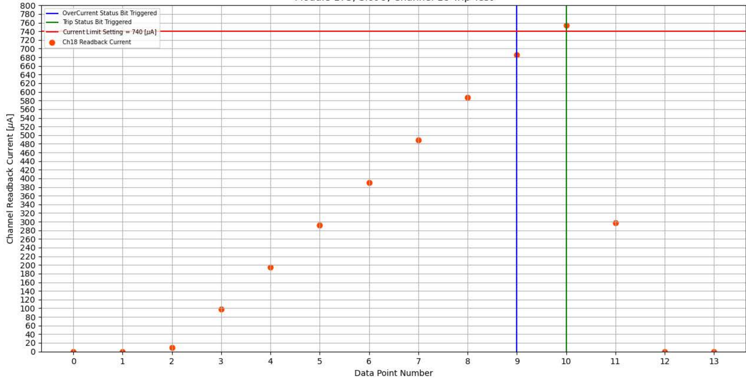
Module 173, Slot 9, Channel 18 Trip Test
