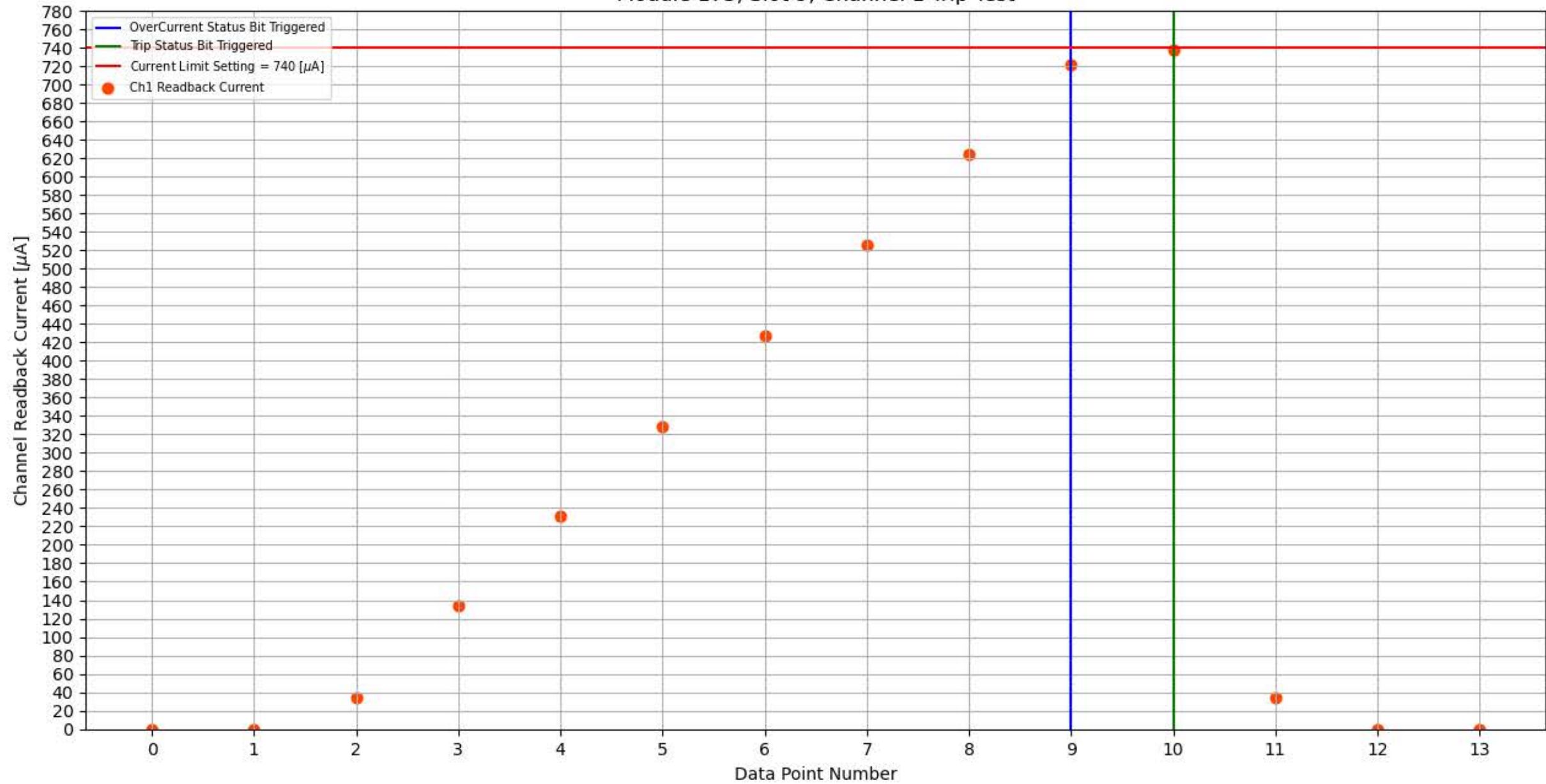
Module 173, Slot 9, Channel 1 Trip Test
