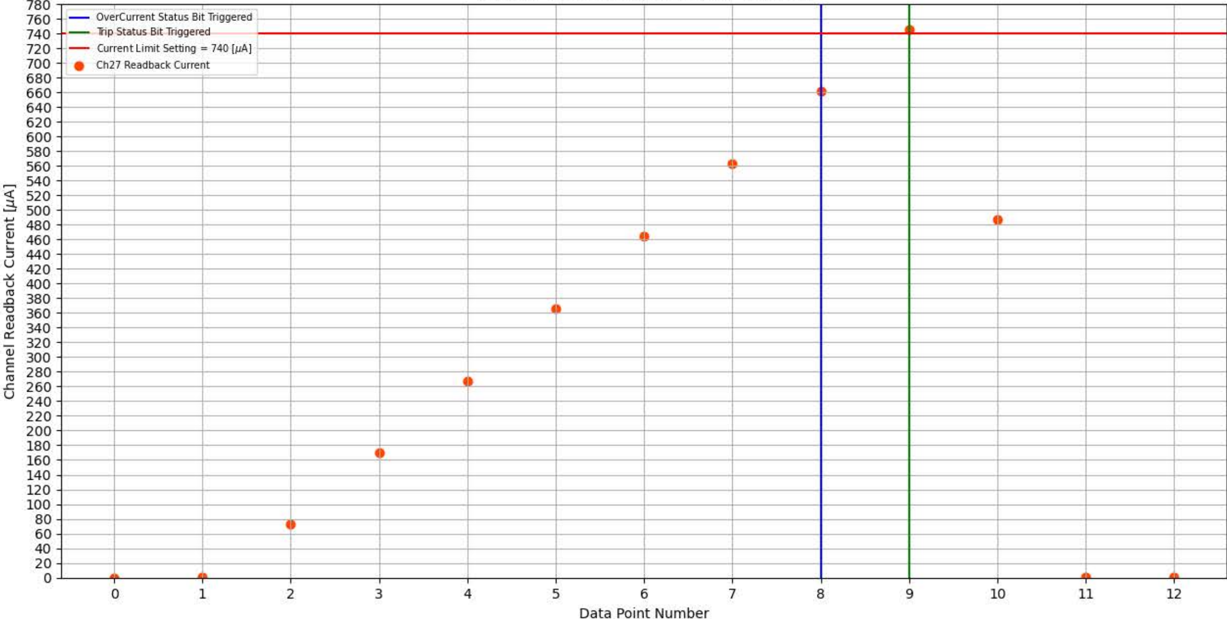
Module 173, Slot 9, Channel 27 Trip Test
