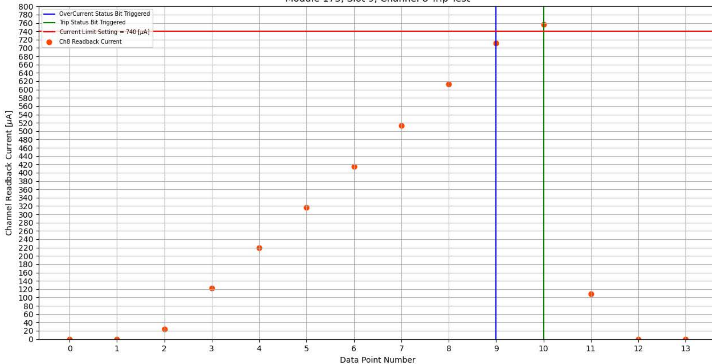
Module 173, Slot 9, Channel 8 Trip Test
