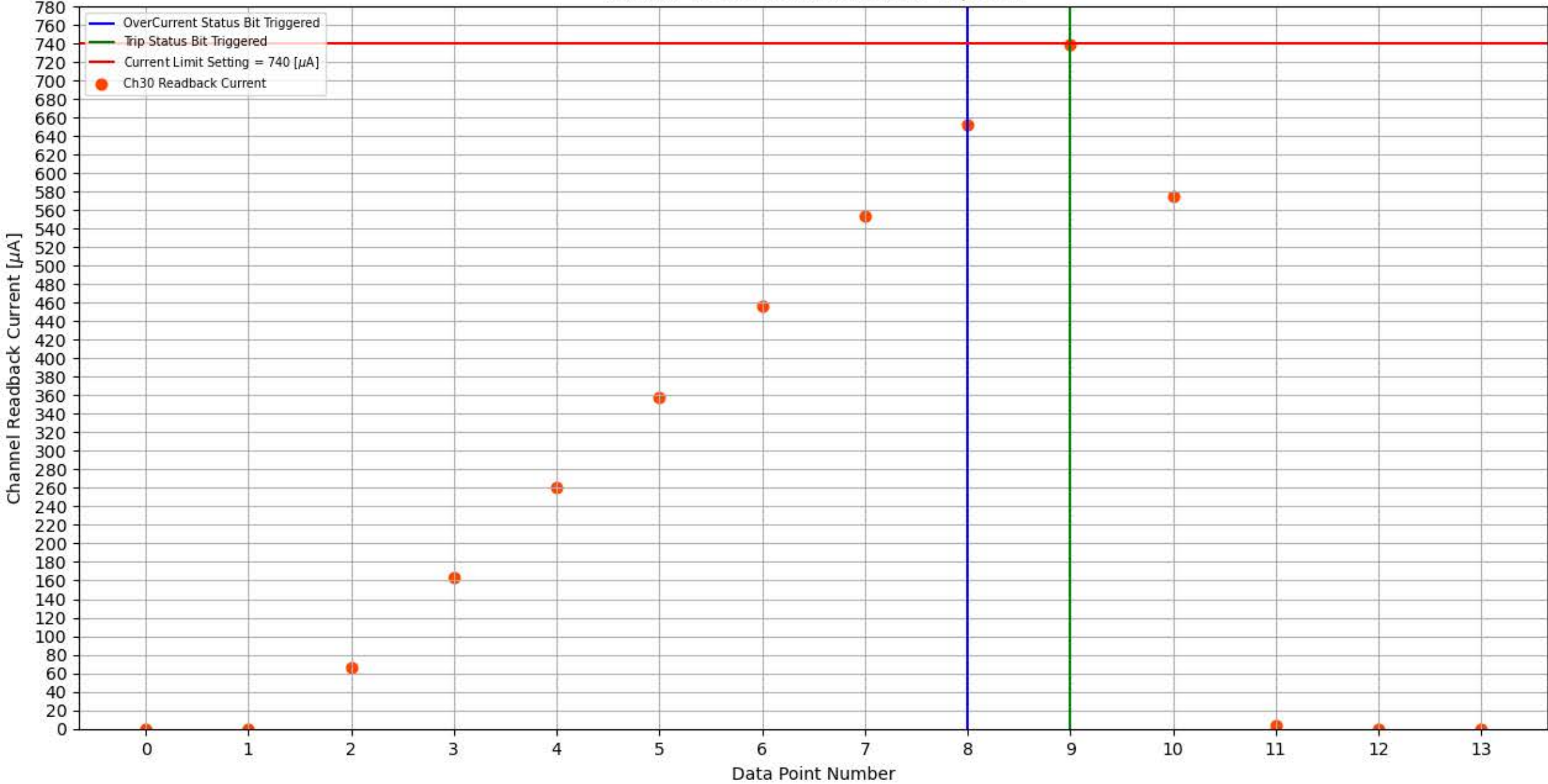
Module 173, Slot 9, Channel 30 Trip Test
