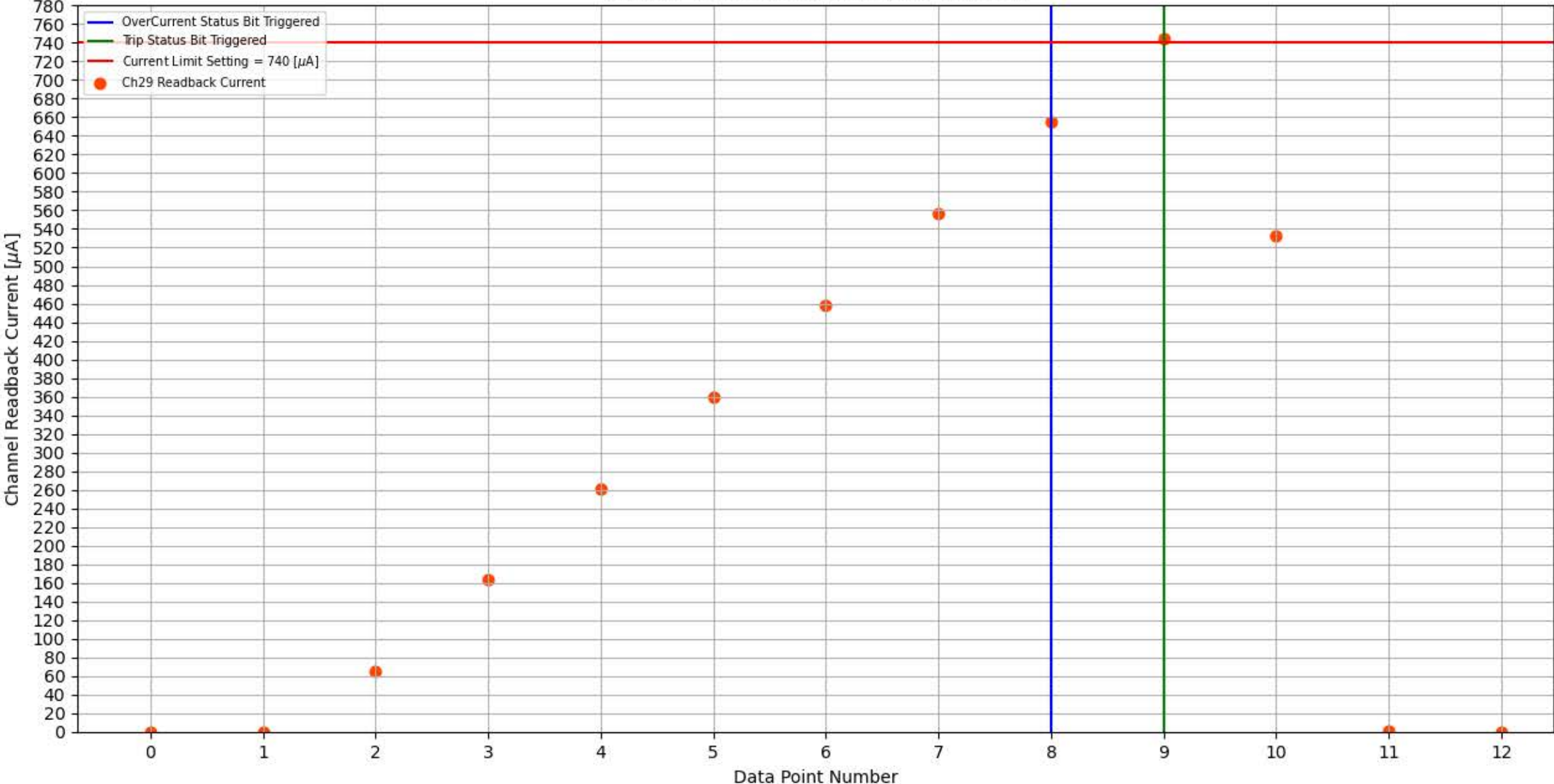
Module 173, Slot 9, Channel 29 Trip Test
