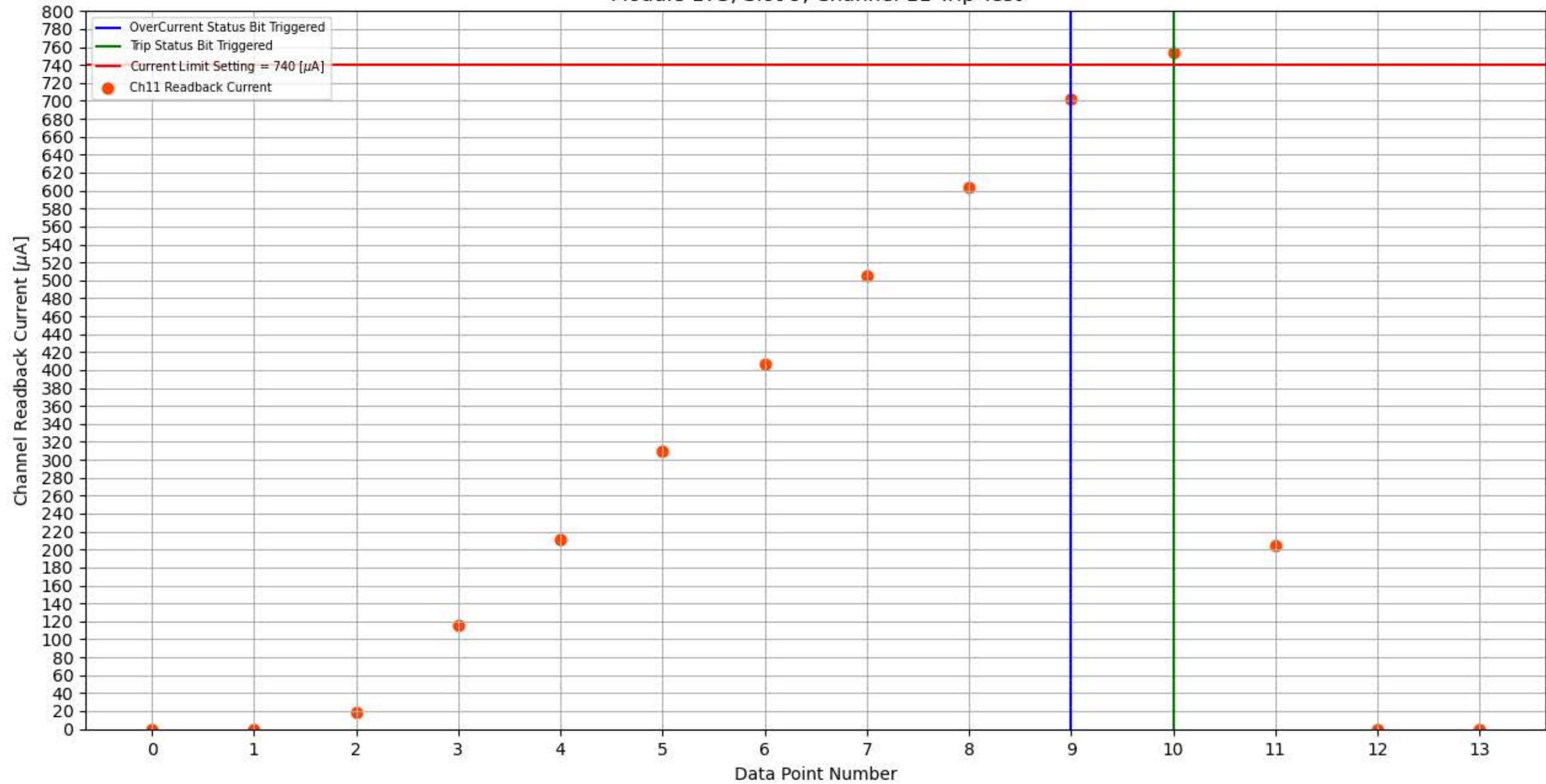
Module 173, Slot 9, Channel 11 Trip Test
