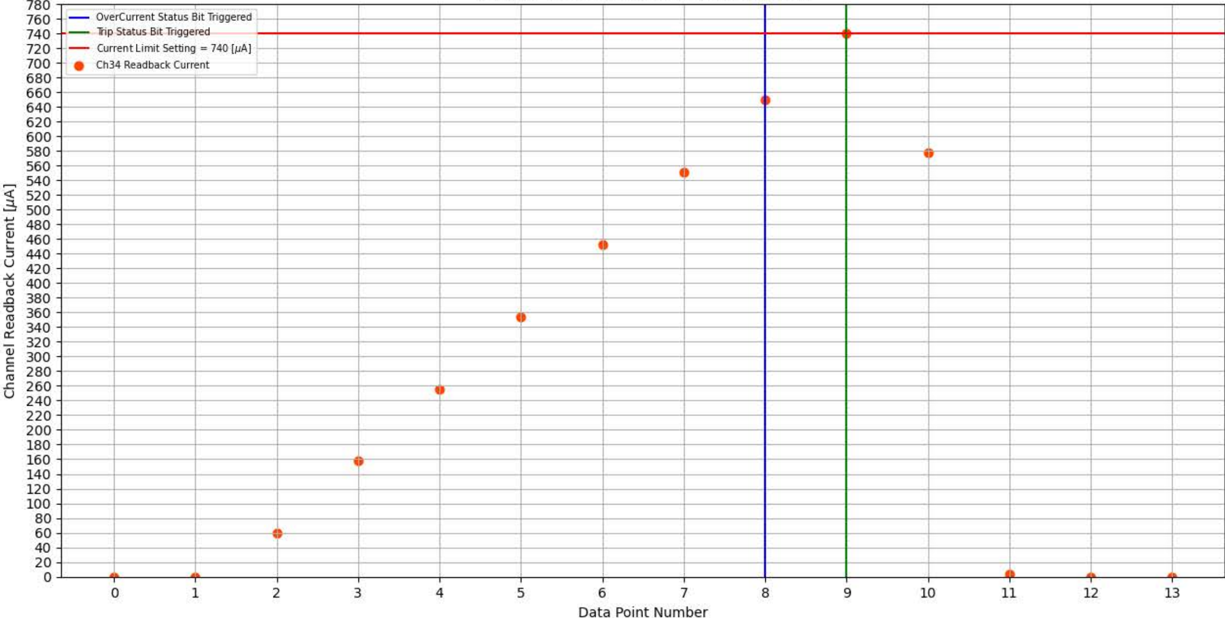
Module 173, Slot 9, Channel 34 Trip Test
