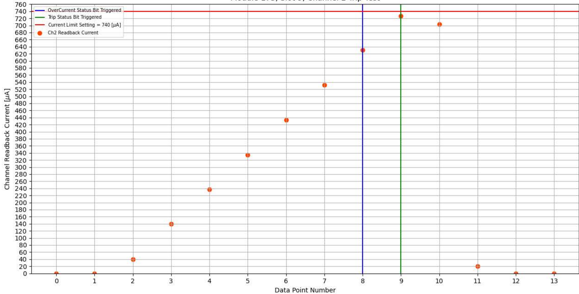
Module 173, Slot 9, Channel 2 Trip Test
