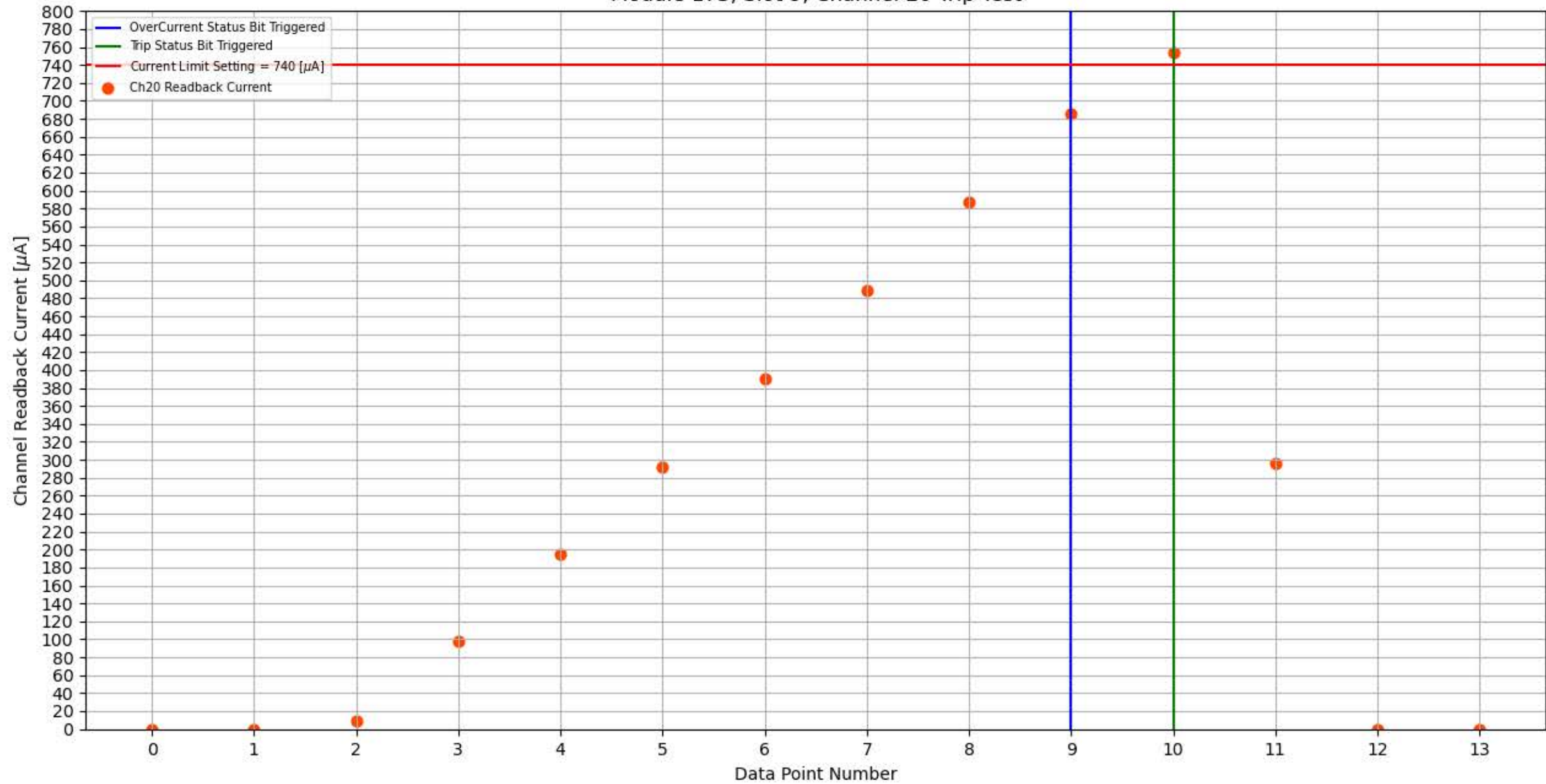
Module 173, Slot 9, Channel 20 Trip Test
