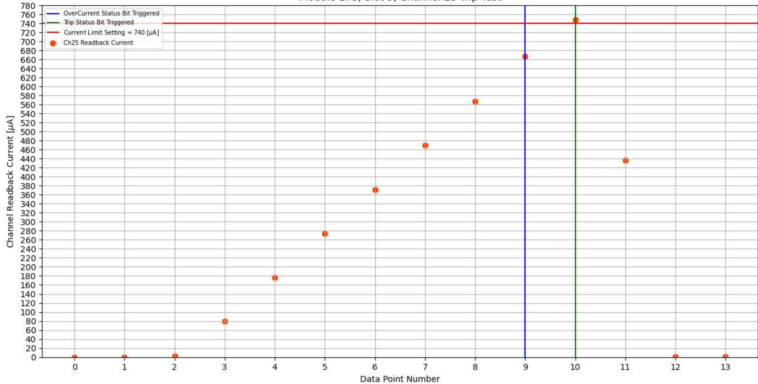
Module 173, Slot 9, Channel 25 Trip Test
