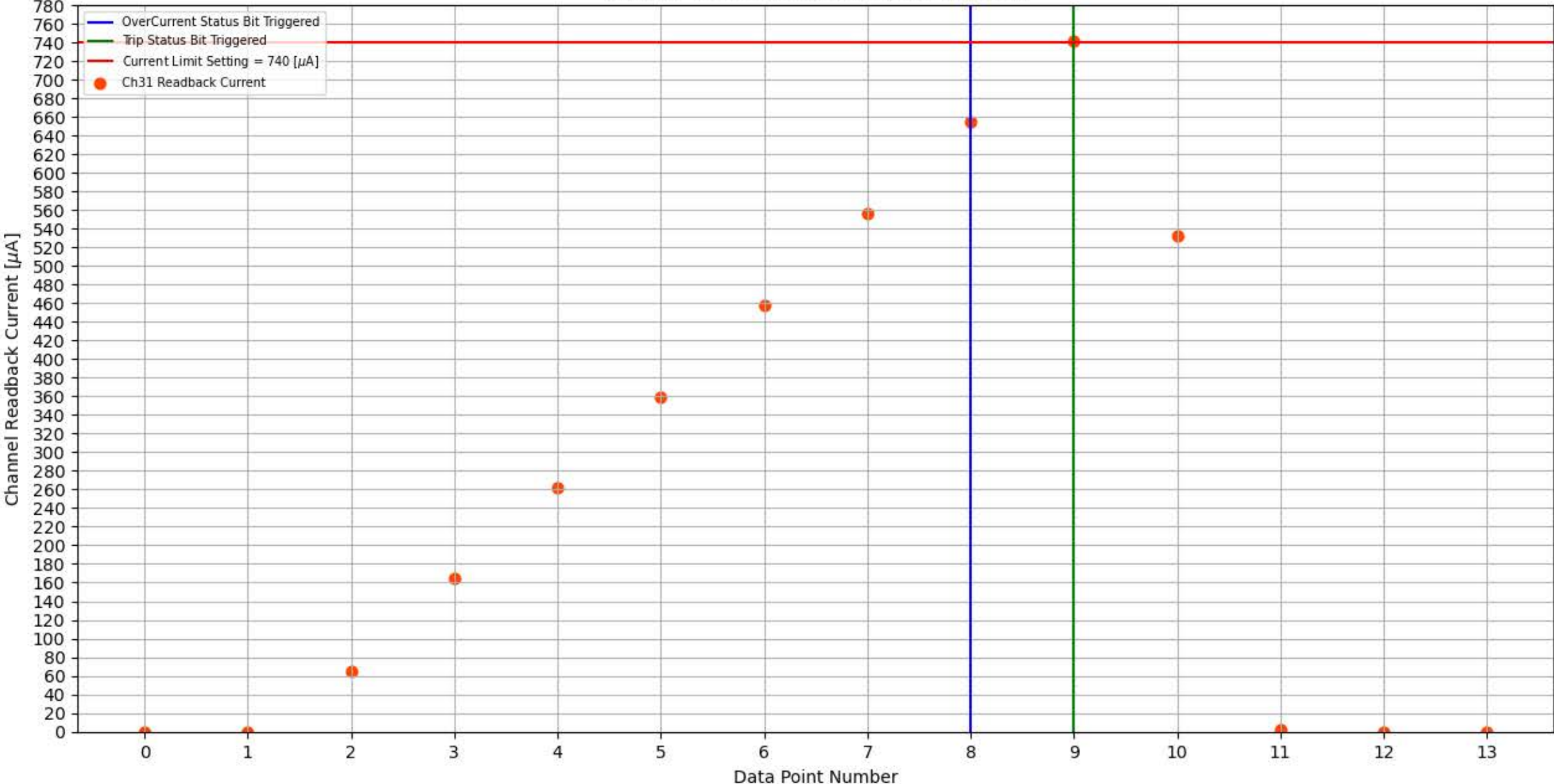
Module 173, Slot 9, Channel 31 Trip Test
