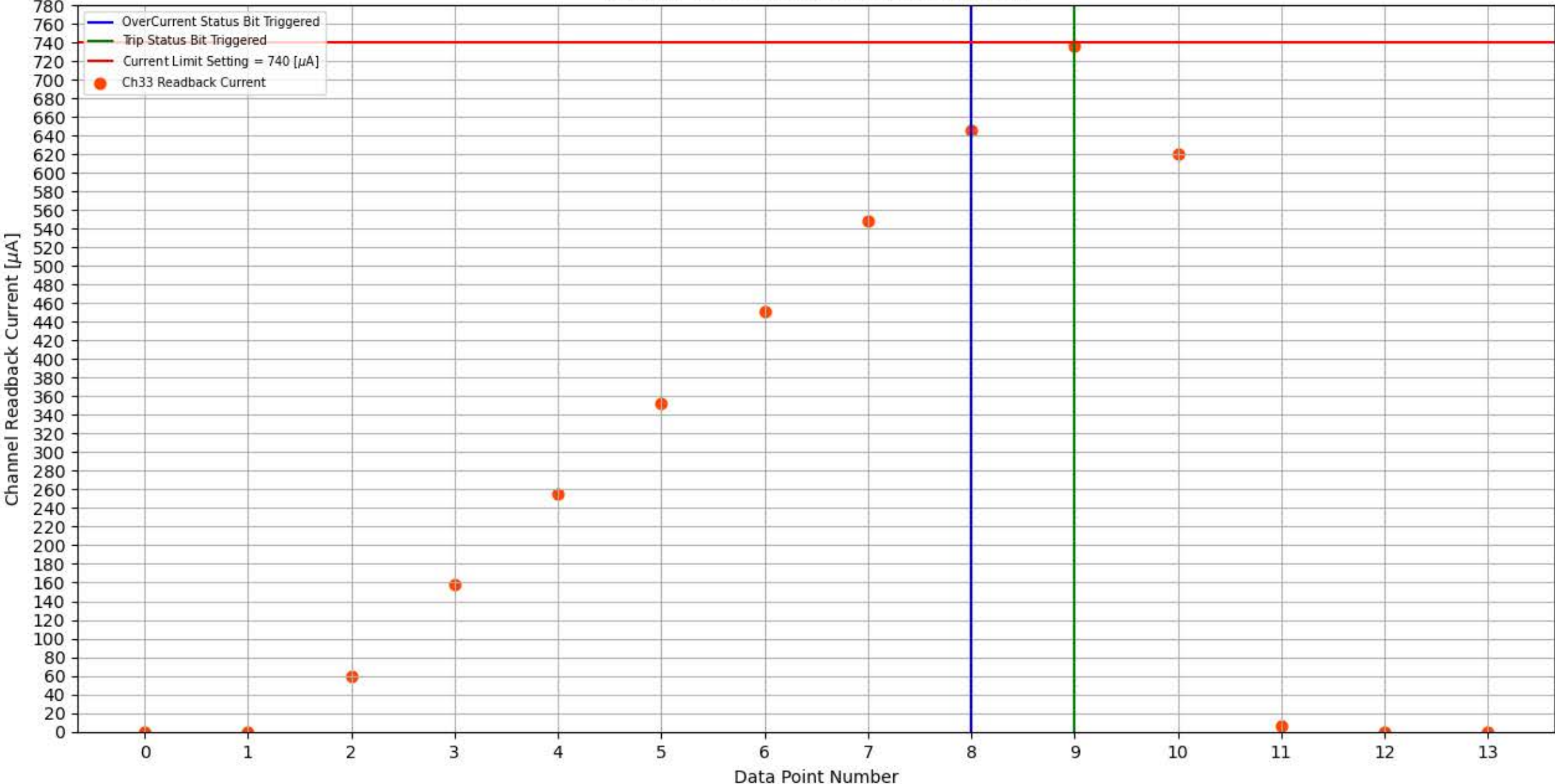
Module 173, Slot 9, Channel 33 Trip Test
