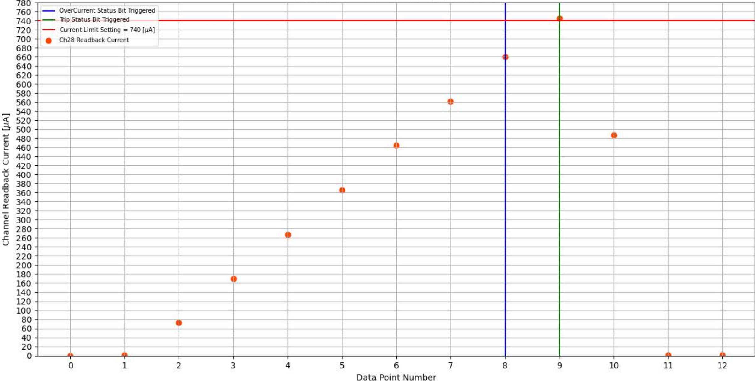
Module 173, Slot 9, Channel 28 Trip Test
