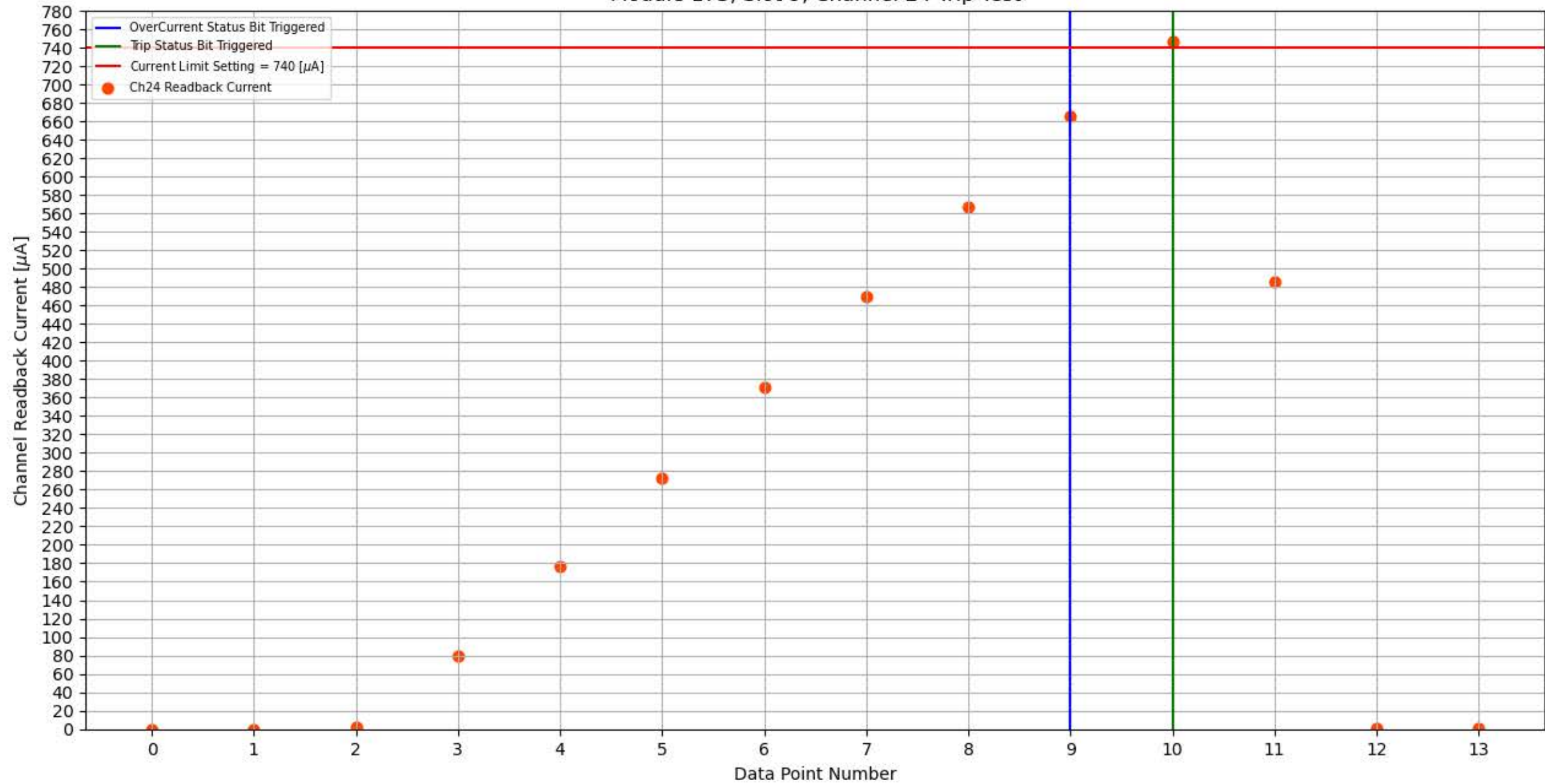
Module 173, Slot 9, Channel 24 Trip Test
