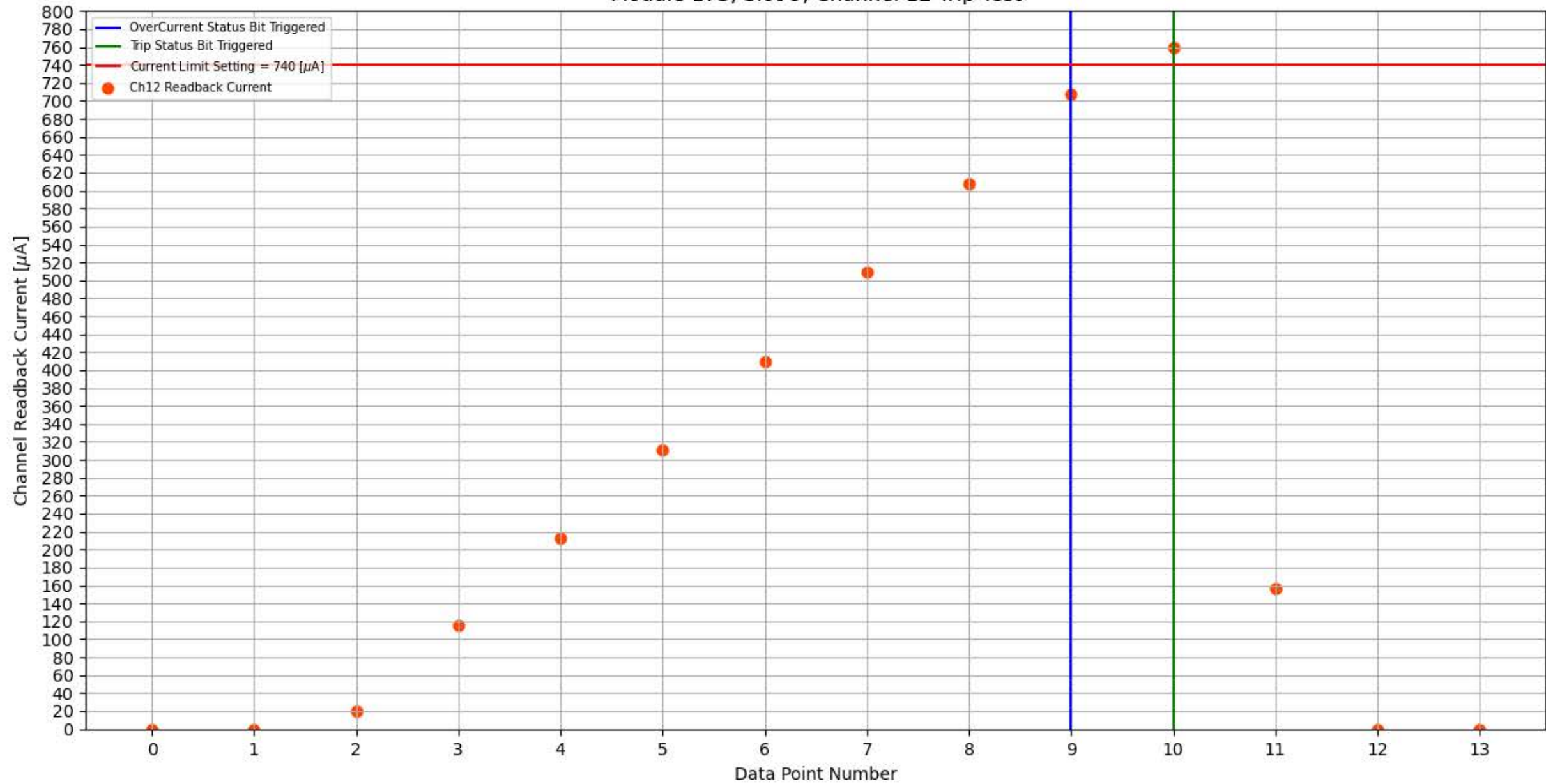
Module 173, Slot 9, Channel 12 Trip Test
