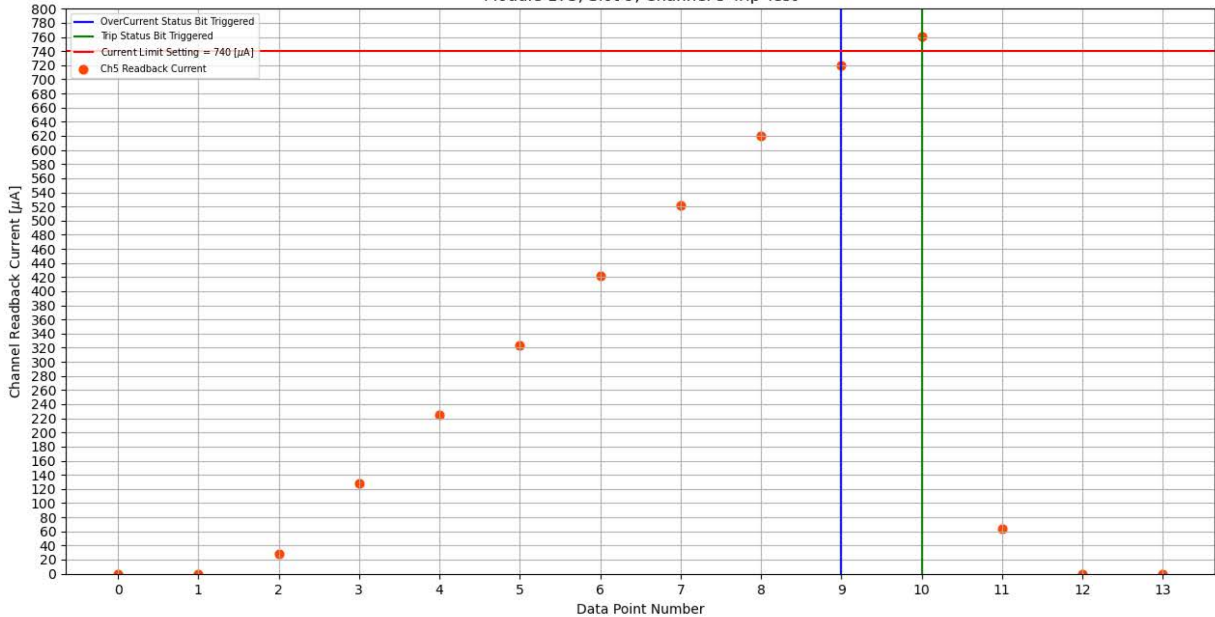
Module 173, Slot 9, Channel 5 Trip Test
