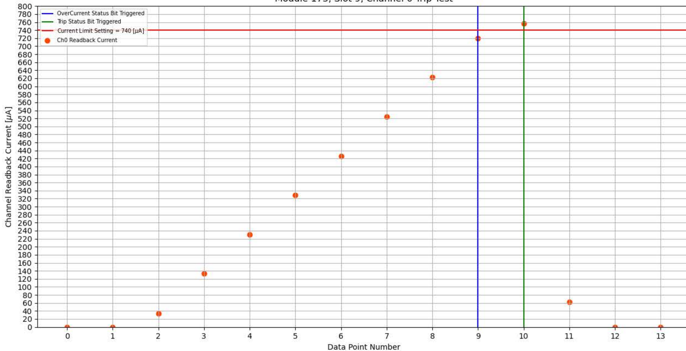
Module 173, Slot 9, Channel 0 Trip Test
