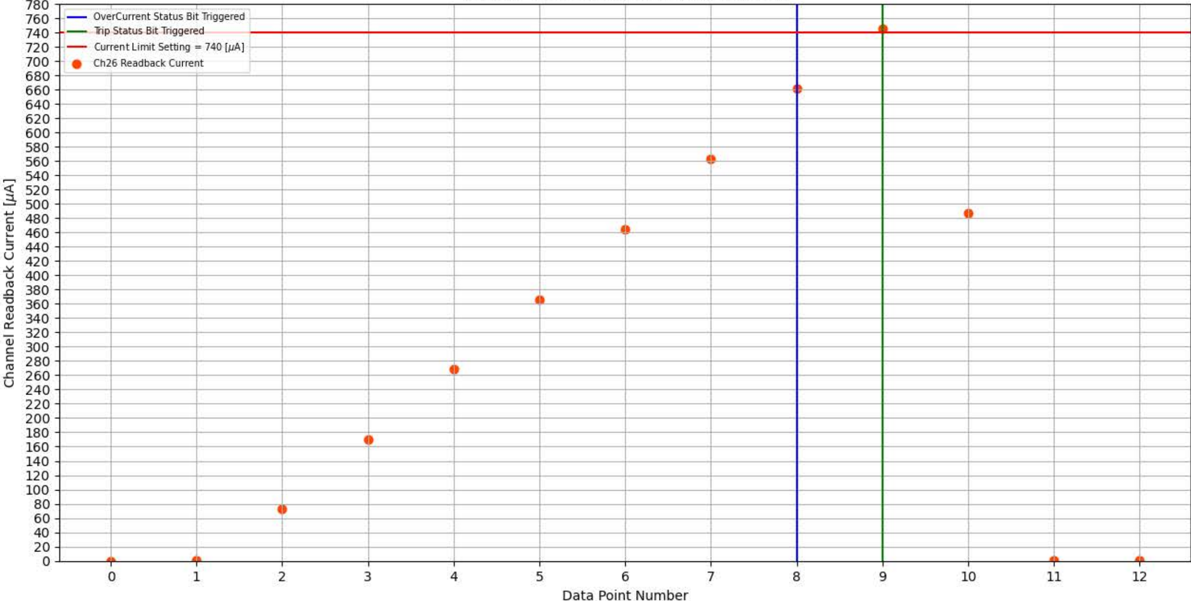
Module 173, Slot 9, Channel 26 Trip Test
