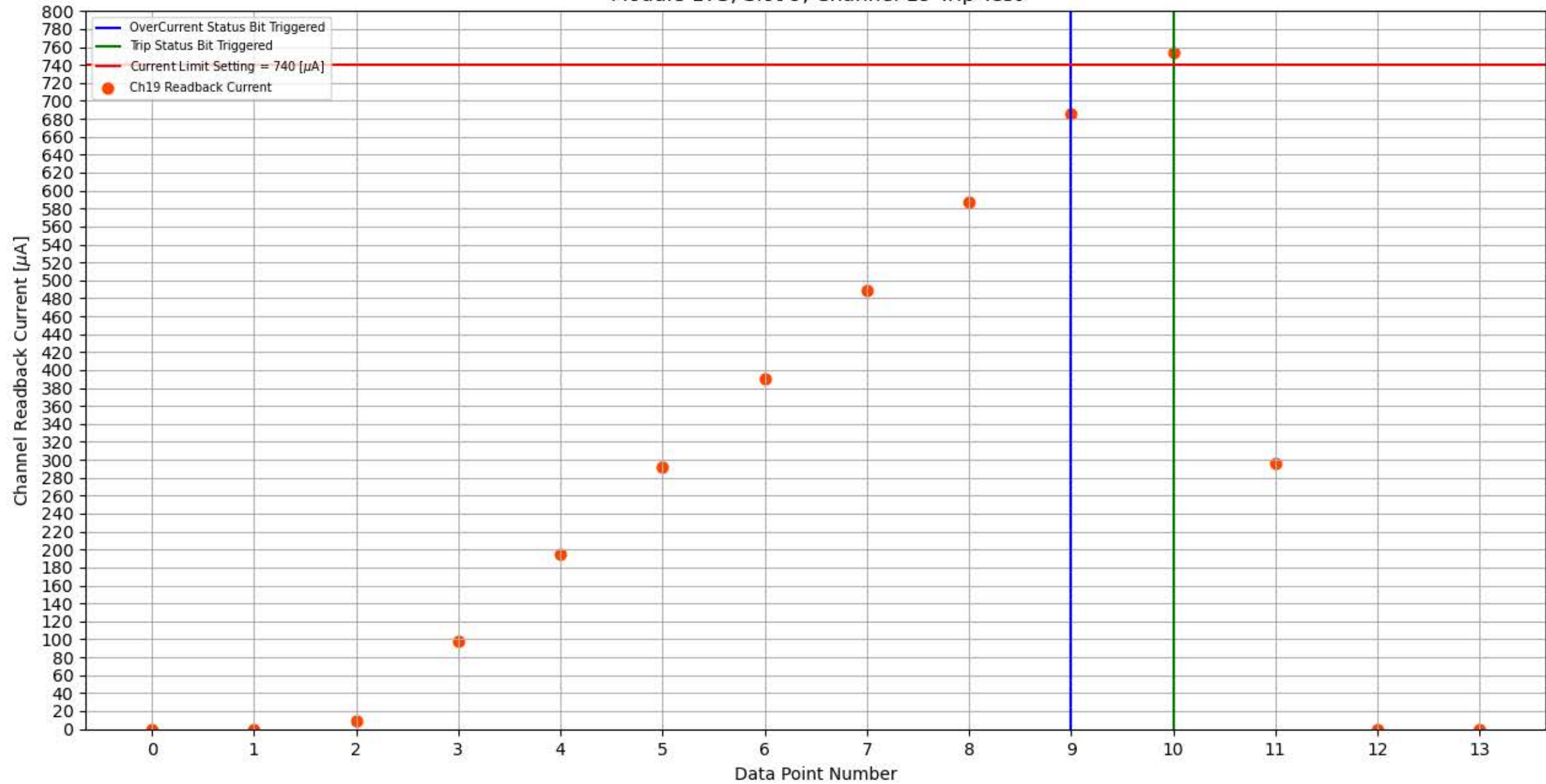
Module 173, Slot 9, Channel 19 Trip Test
