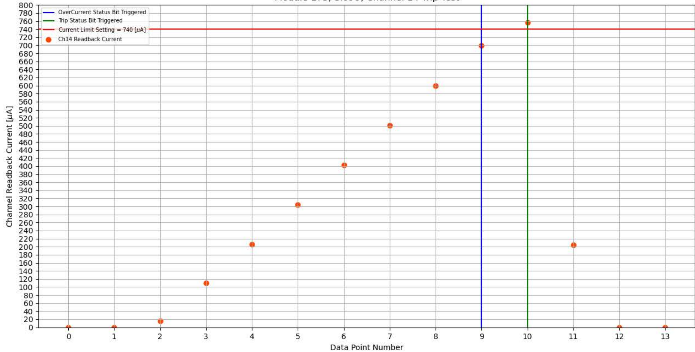
Module 173, Slot 9, Channel 14 Trip Test
