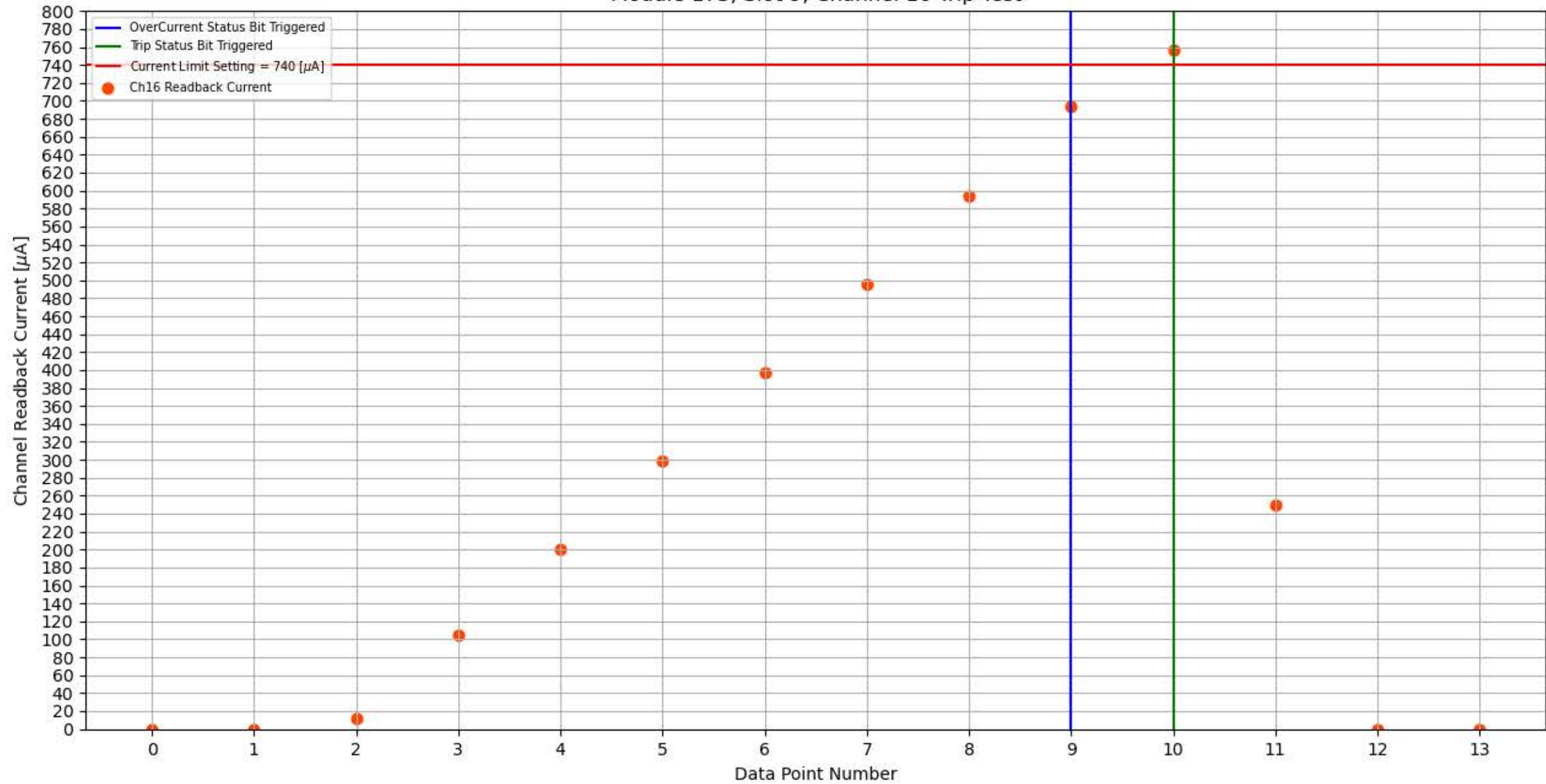
Module 173, Slot 9, Channel 16 Trip Test
