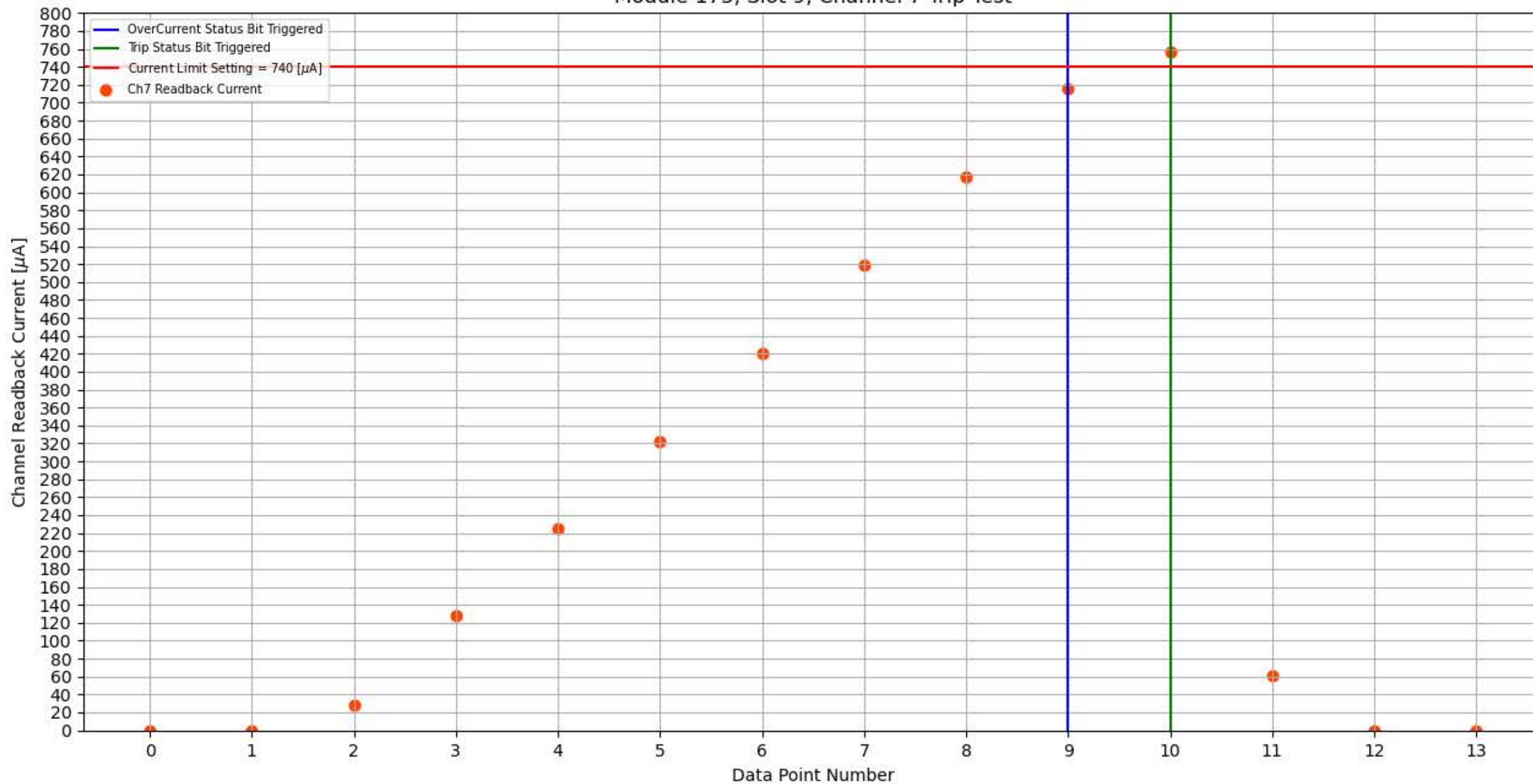
Module 173, Slot 9, Channel 7 Trip Test
