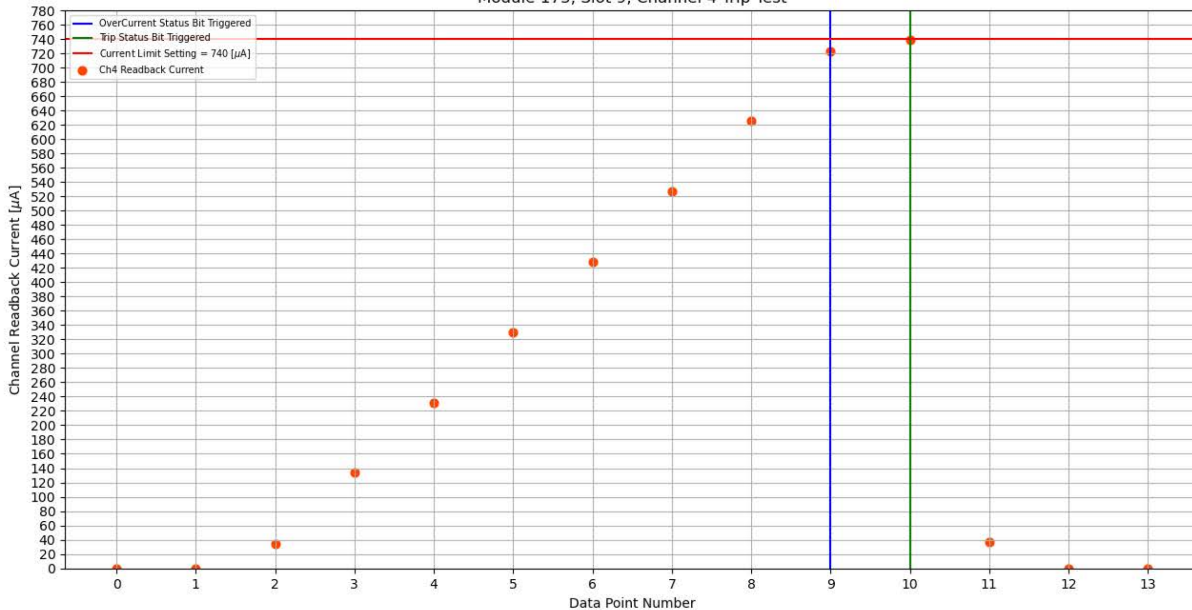
Module 173, Slot 9, Channel 4 Trip Test
