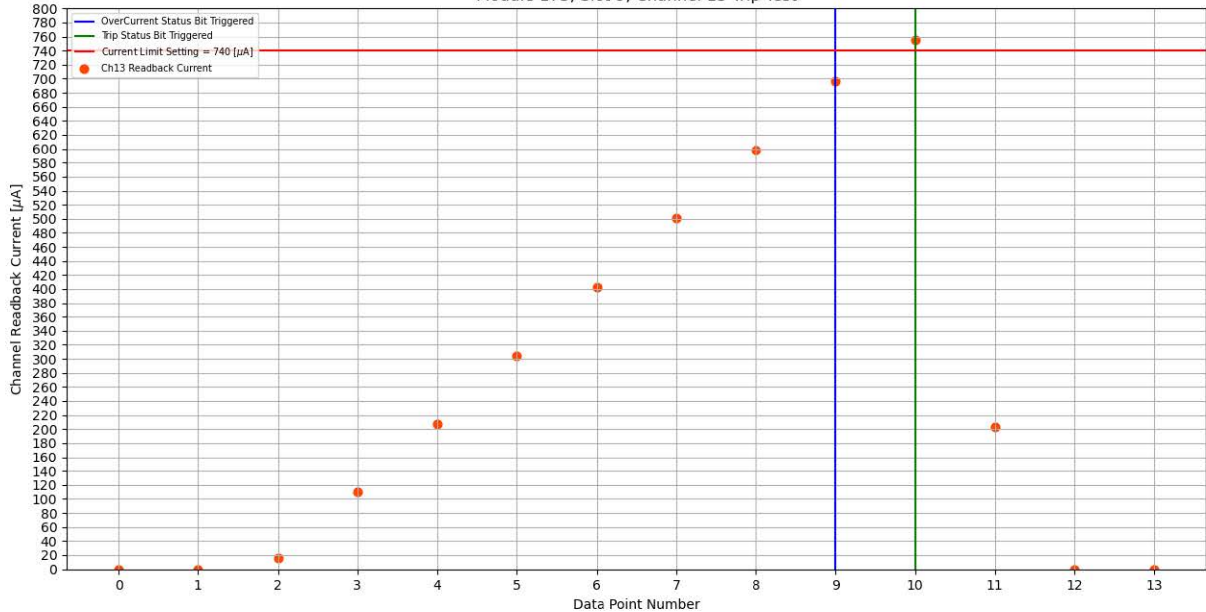
Module 173, Slot 9, Channel 13 Trip Test
