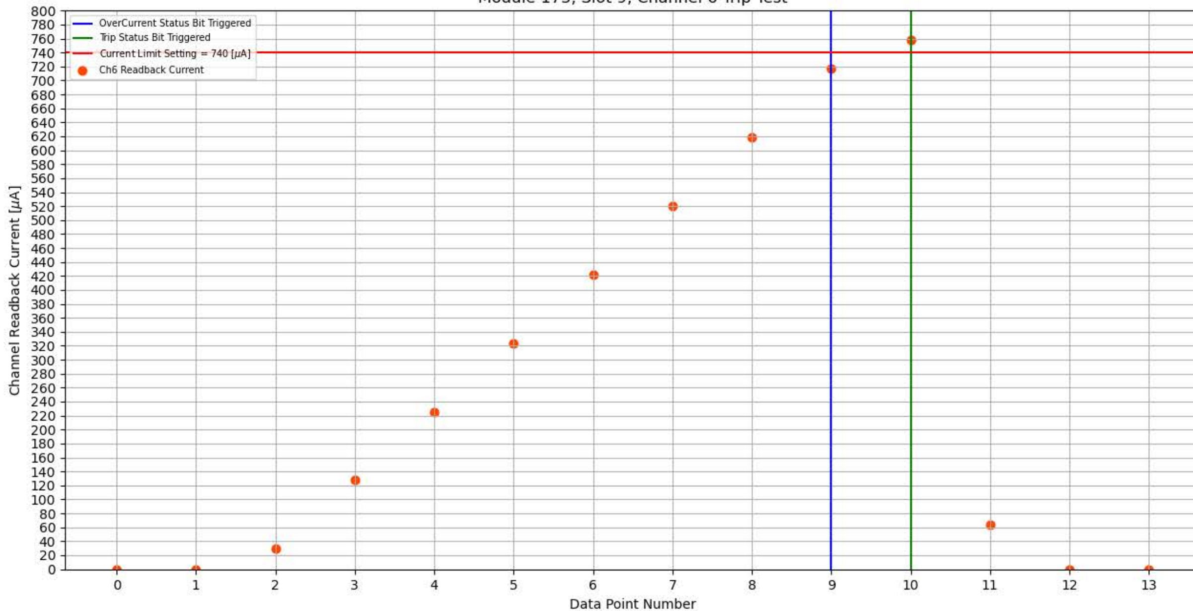
Module 173, Slot 9, Channel 6 Trip Test
